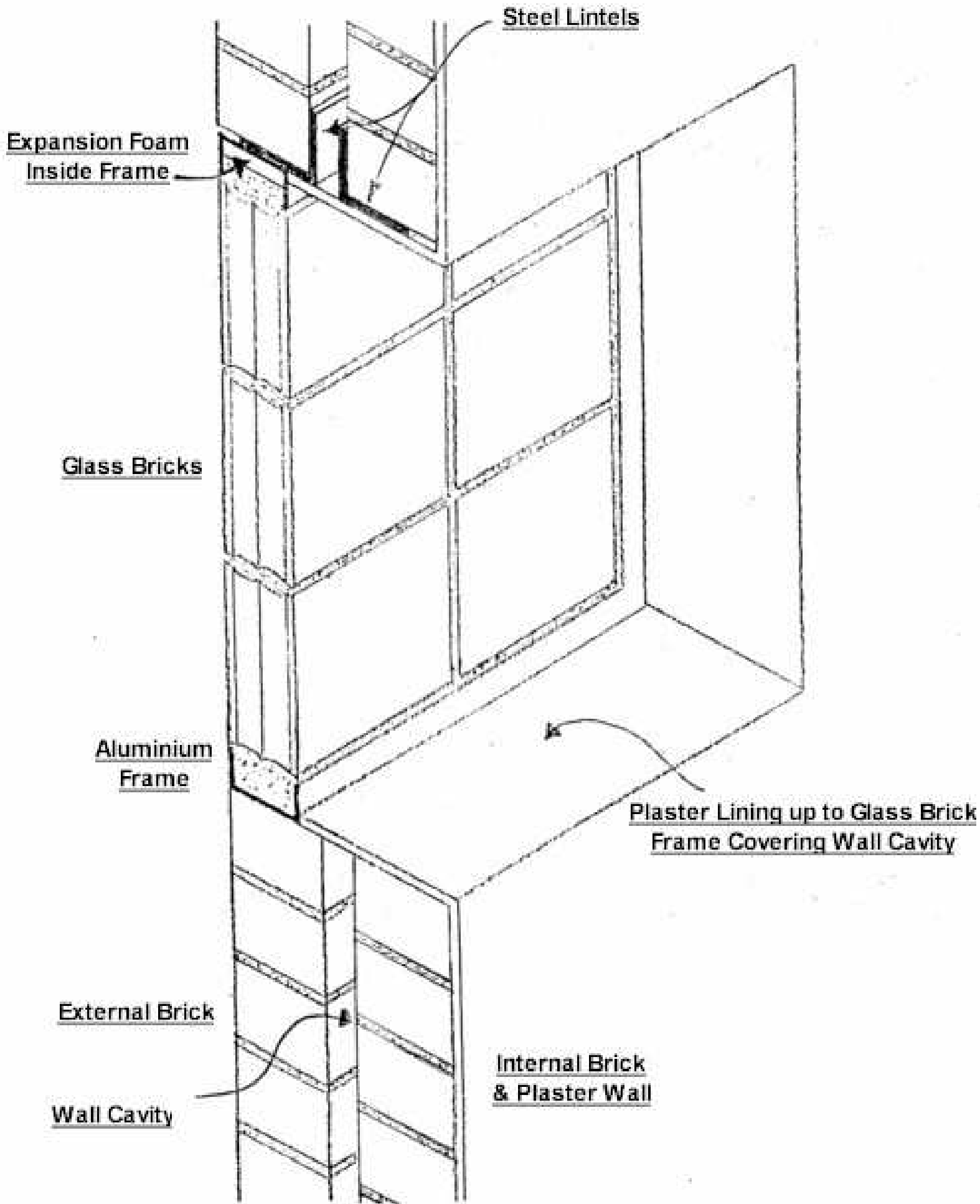
SECTION THROUGH SOLID BRICK WALL
